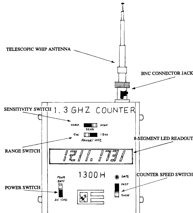
Figure 17. An Optoelectronics 1300H hand-held frequency counter (0-1300 MHz).
