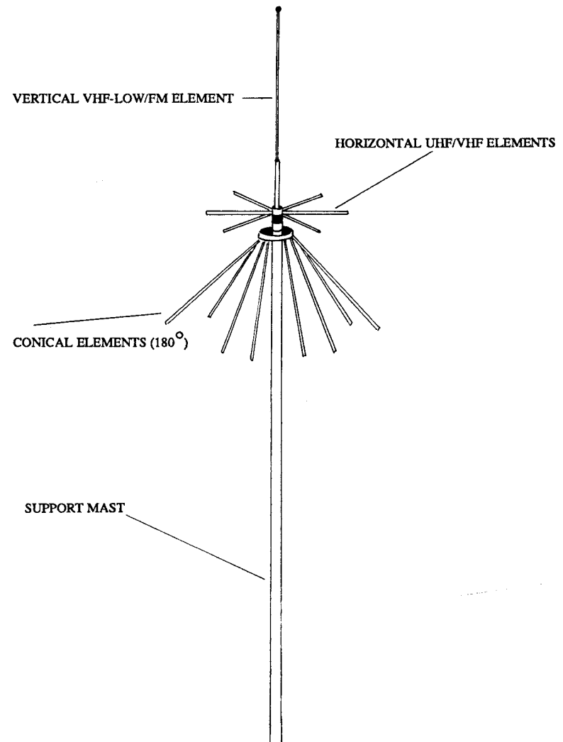
Figure 10. An ICOM model AH-7000 discone antenna with fifteen elements (25-2000 MHz). This omnidirectional, high-gain antenna can transmit and receive on VHF and UHF frequencies.
